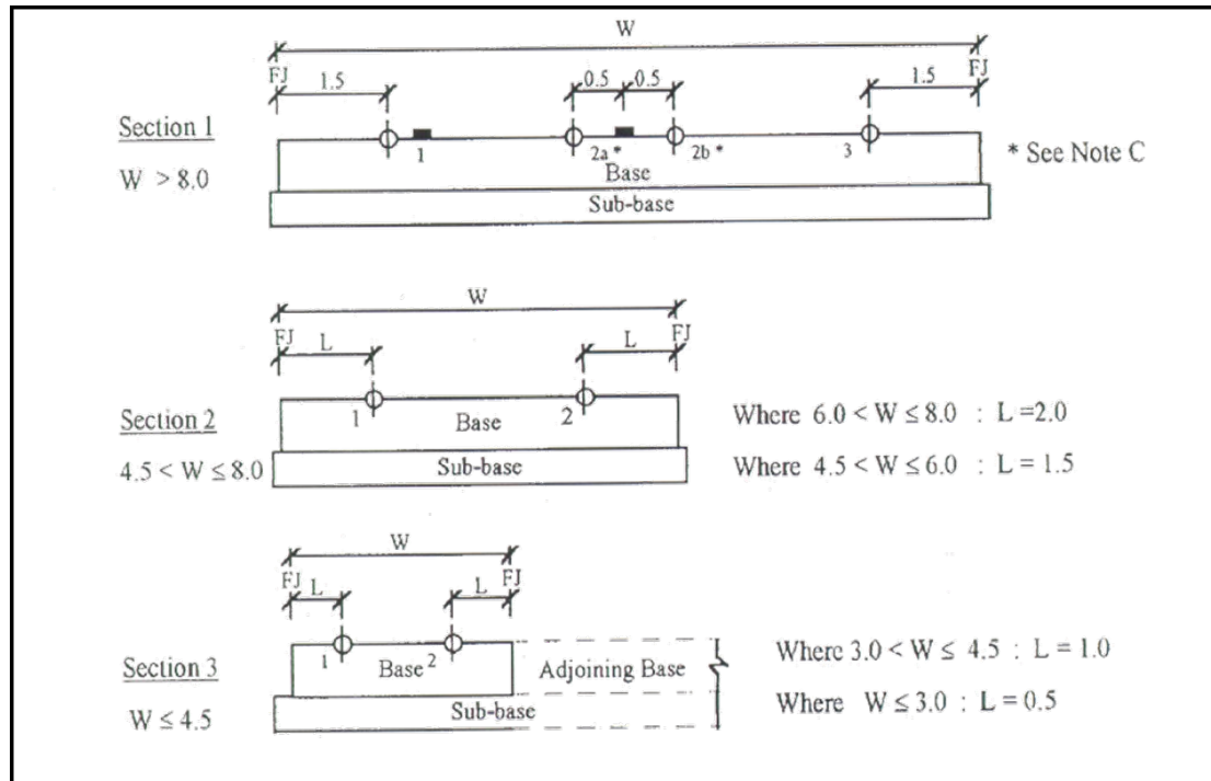
Figure 12.3.3 – Survey height cross-sections
