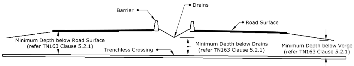
Figure 5.2.2(b) – Minimum depth below dual carriageway
